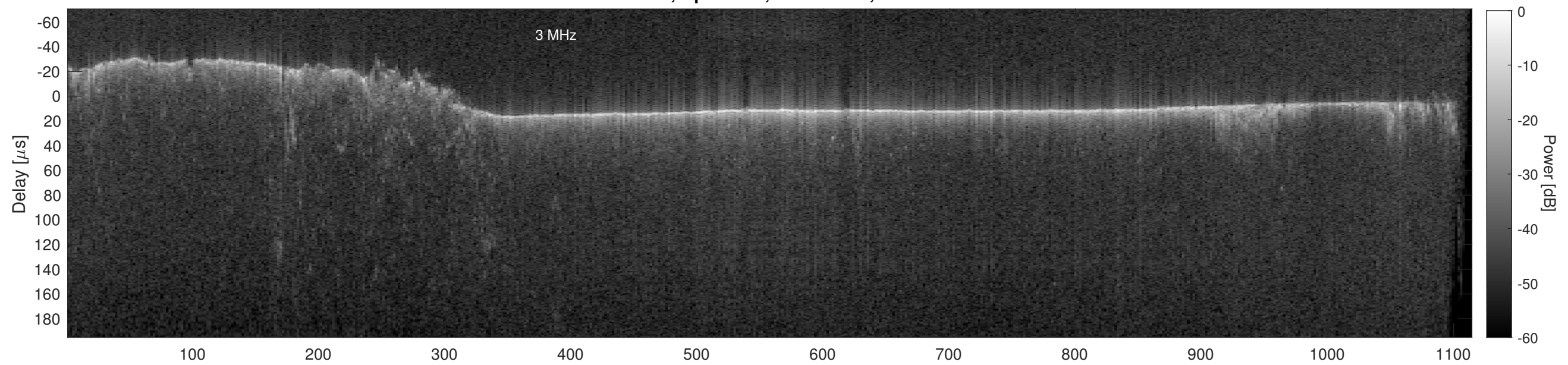
Orbit 22737, Cluttergram
