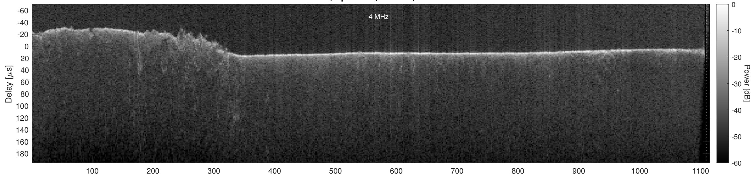
Orbit 22737, Optimized, Window, Channel 2
