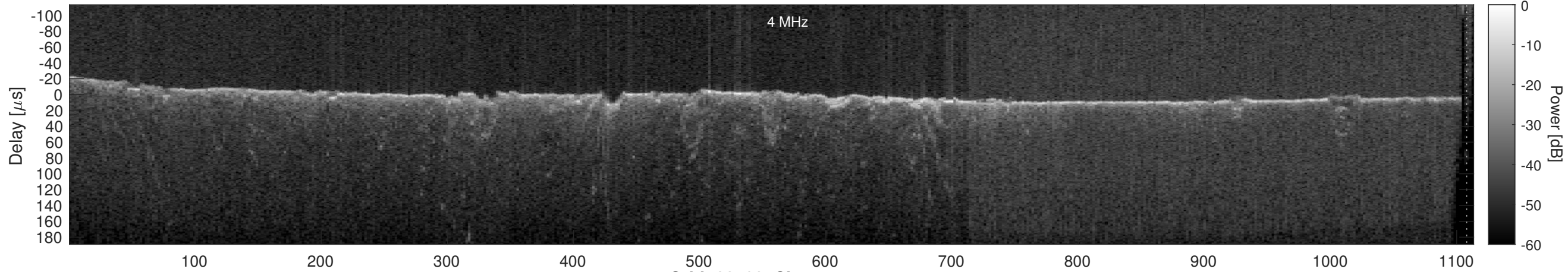
Orbit 22738, Cluttergram
