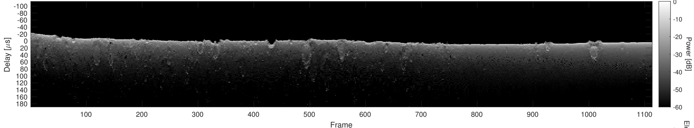
Orbit 22738, Cluttergram
