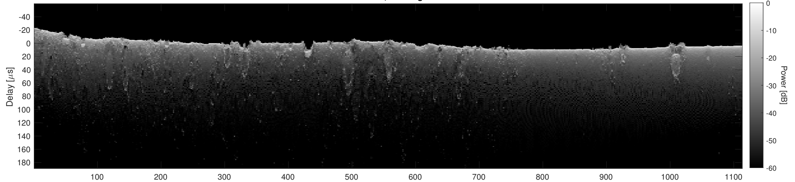
Orbit 22738, Cluttergram
