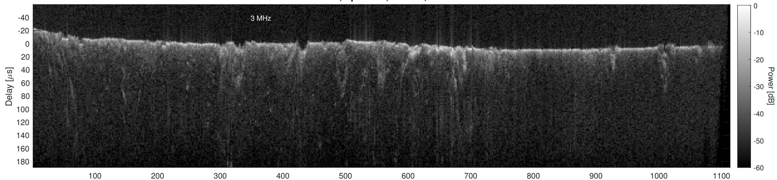
Orbit 22738, Cluttergram
