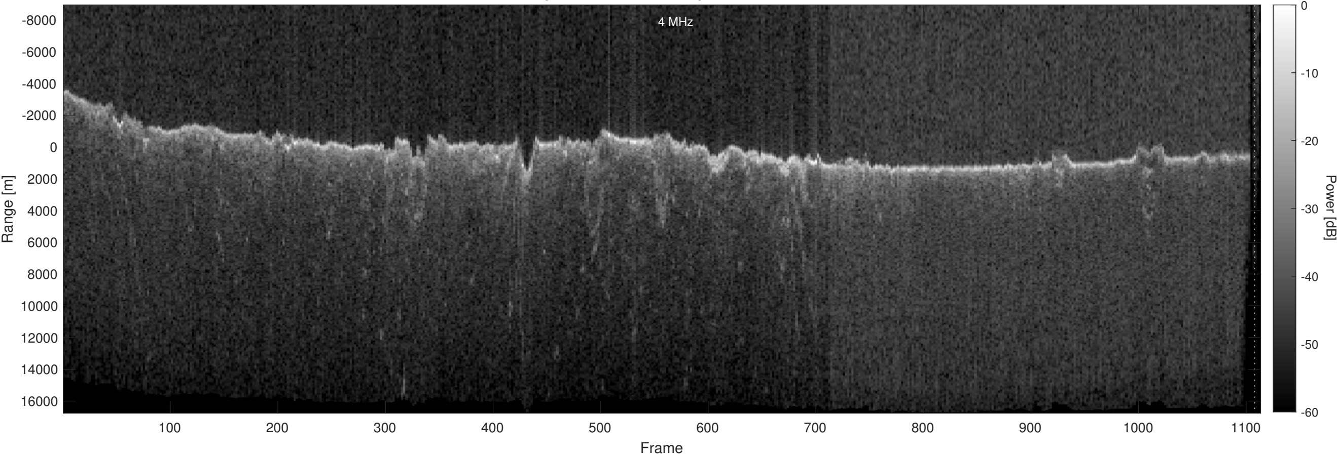
Orbit 22738, Optimized, Window, Depth-Corrected, Channel 2
