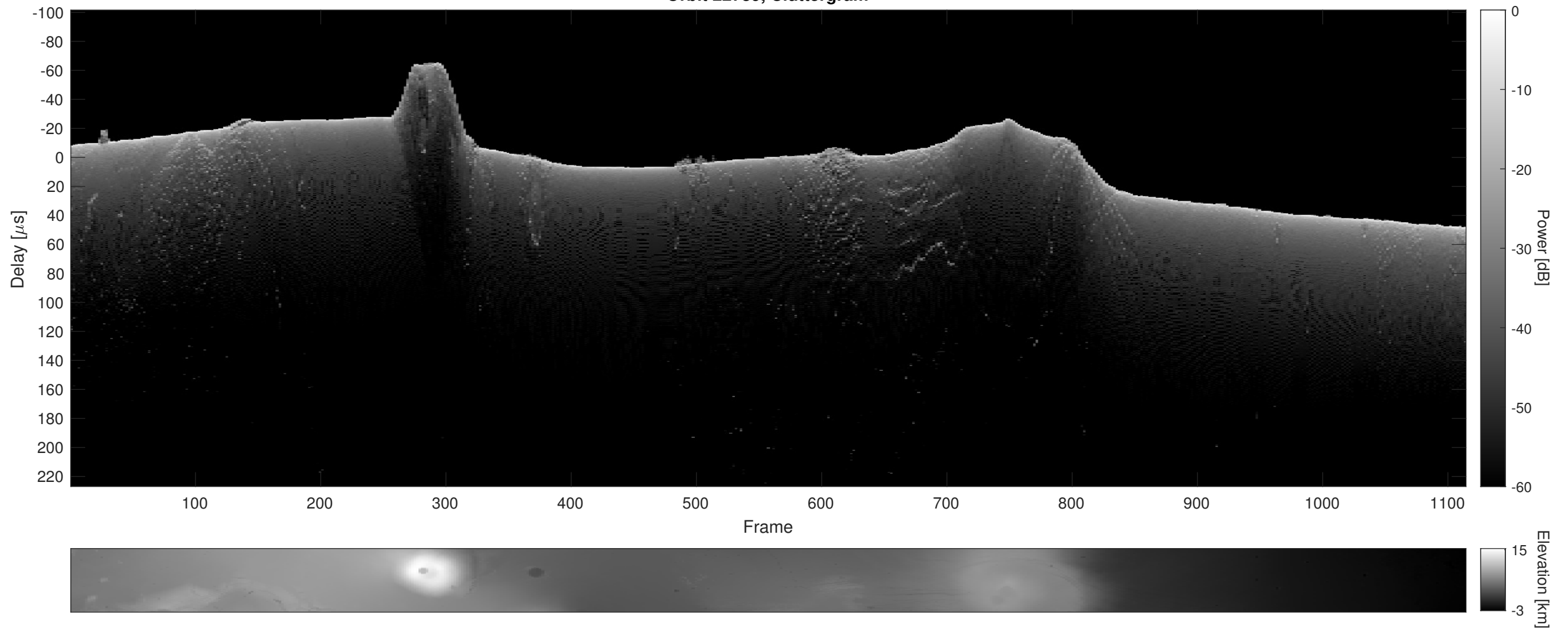
Orbit 22739, Cluttergram
