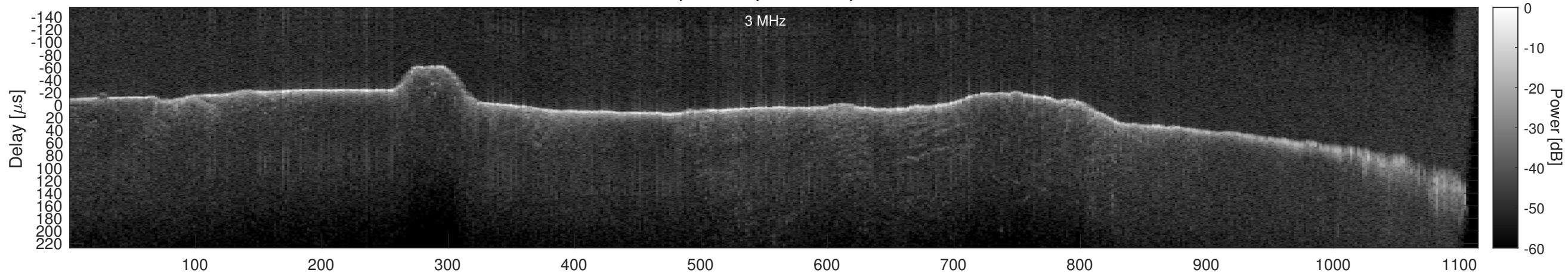
Orbit 22739, Window, Channel 2, Chapman
