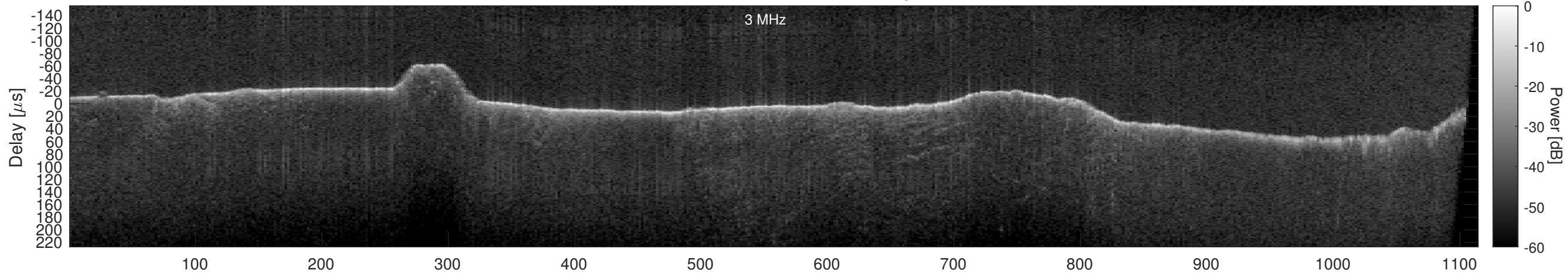
Orbit 22739, Window, Channel 2, Optimized
