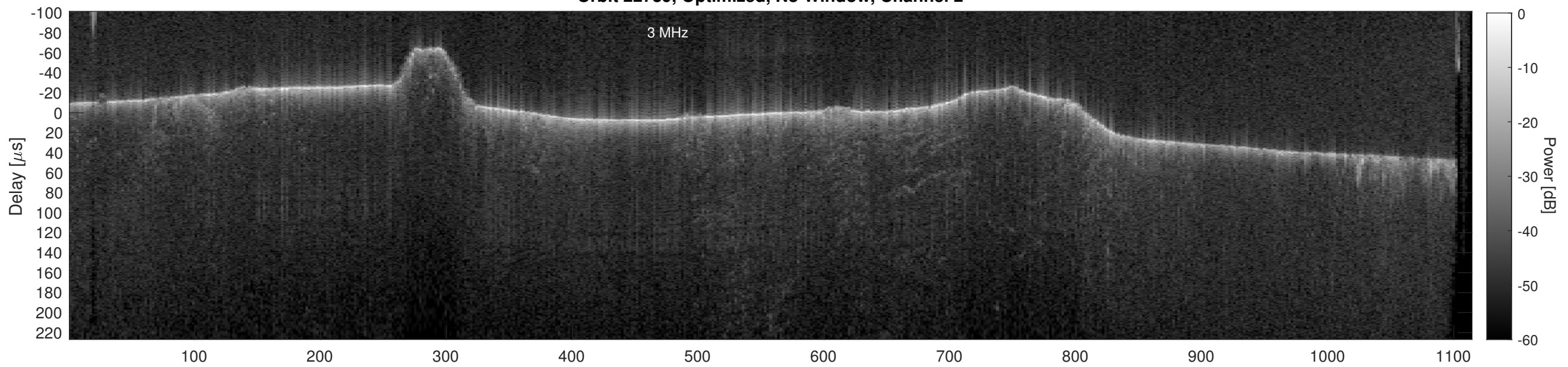
Orbit 22739, Cluttergram
