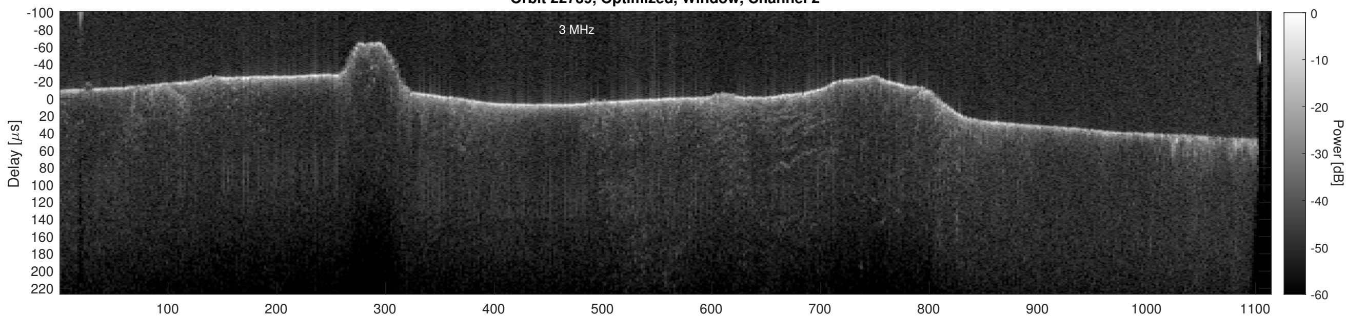
Orbit 22739, Cluttergram
