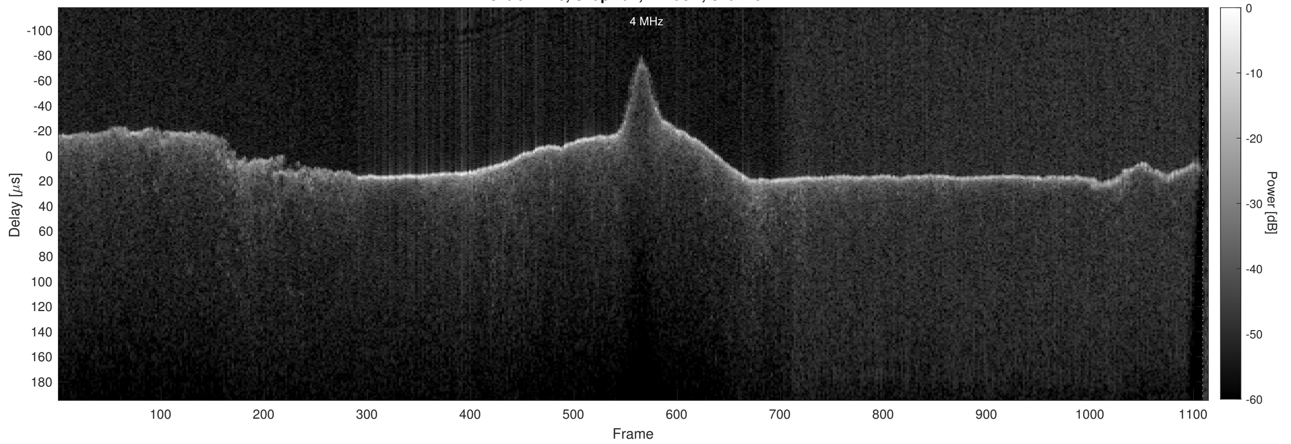
Orbit 22740, Chapman, Window, Channel 2
