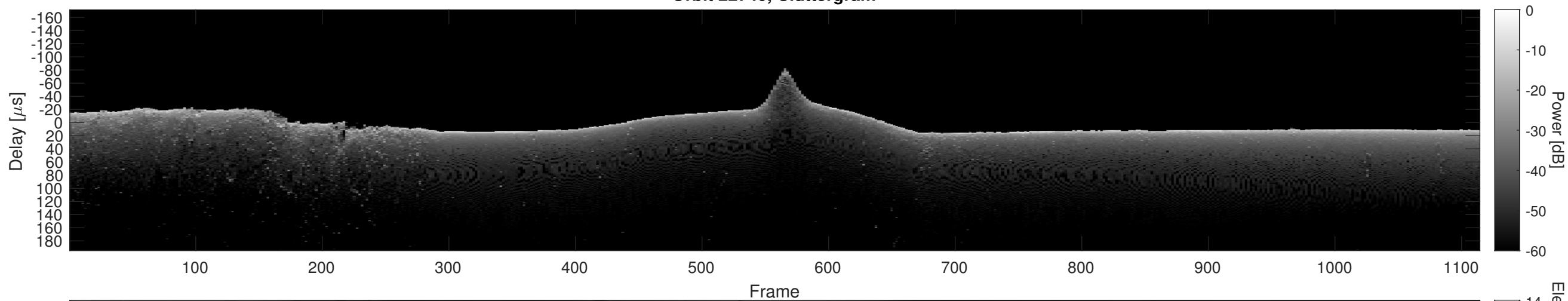
Orbit 22740, Cluttergram
