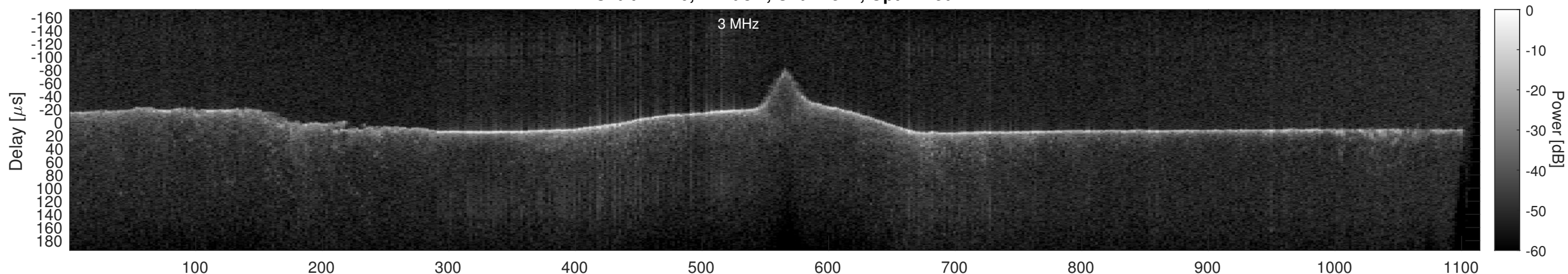
Orbit 22740, Cluttergram
