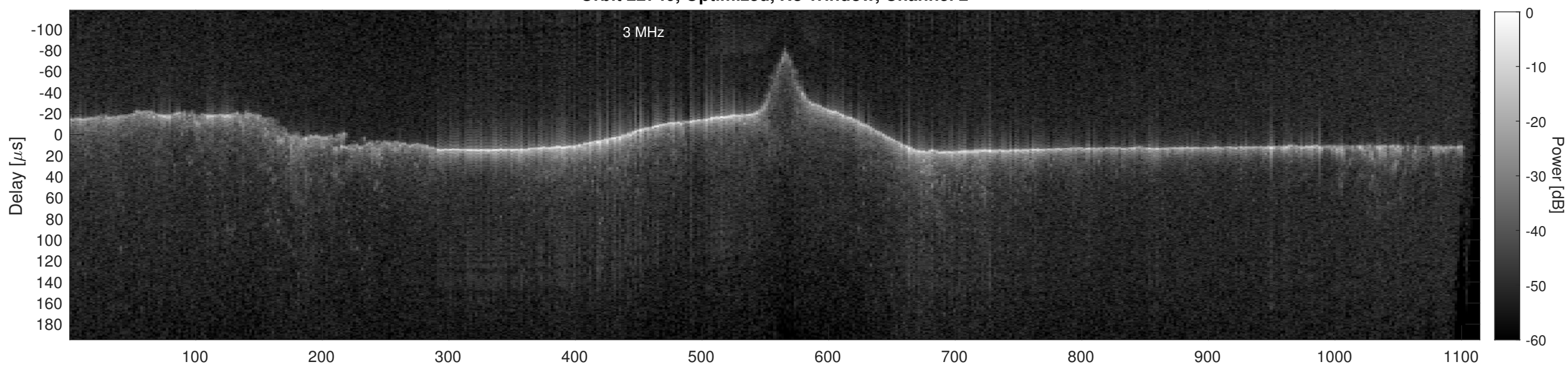
Orbit 22740, Cluttergram
