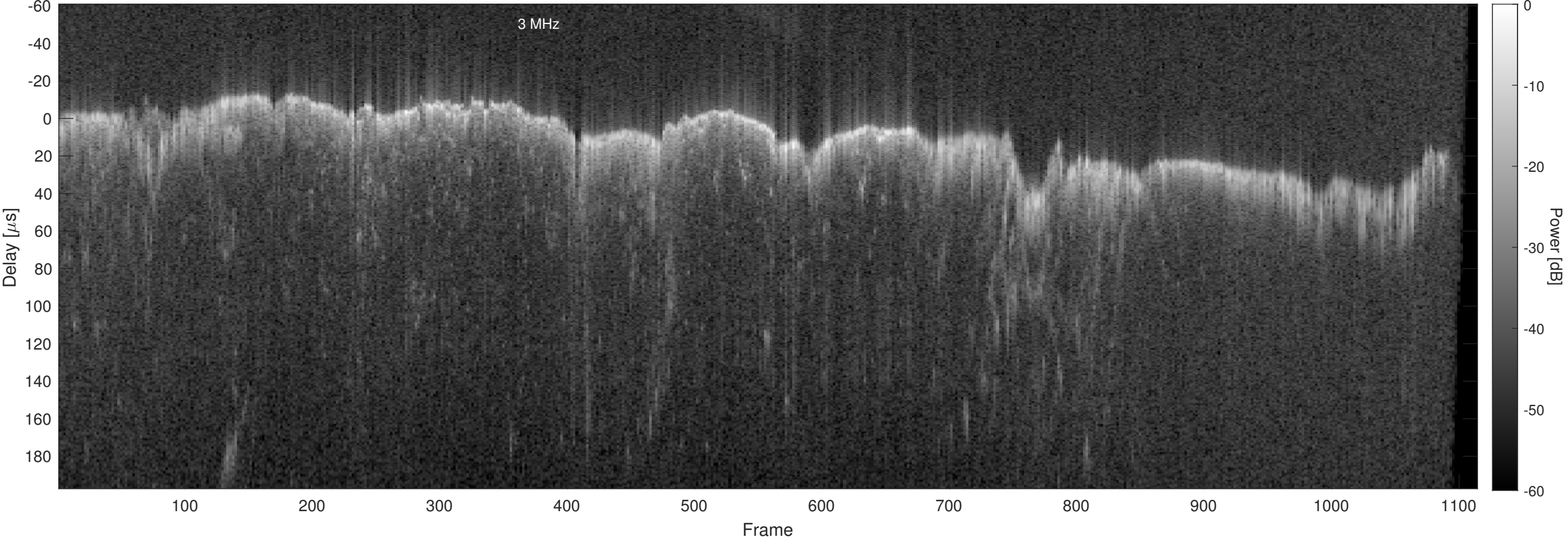
Orbit 22741, Chapman, No Window, Channel 2
