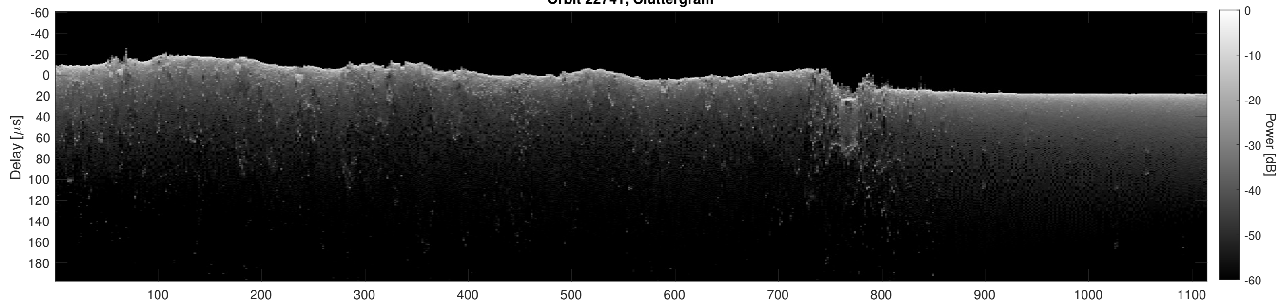
Orbit 22741, Cluttergram
