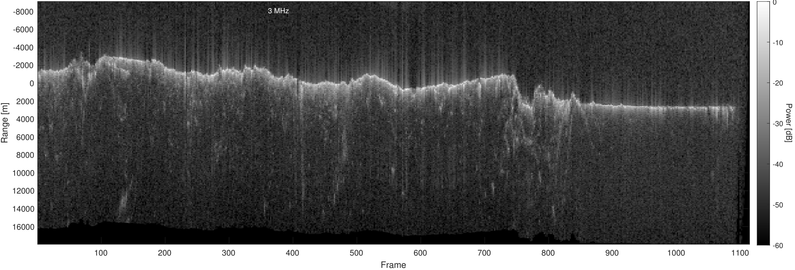
Orbit 22741, Optimized, No Window, Depth-Corrected, Channel 2
