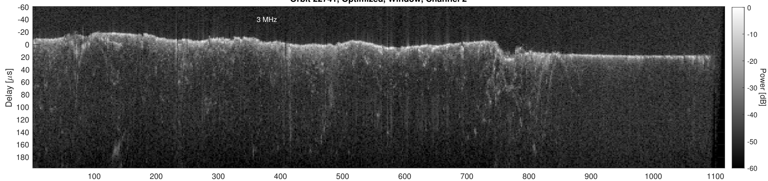
Orbit 22741, Cluttergram
