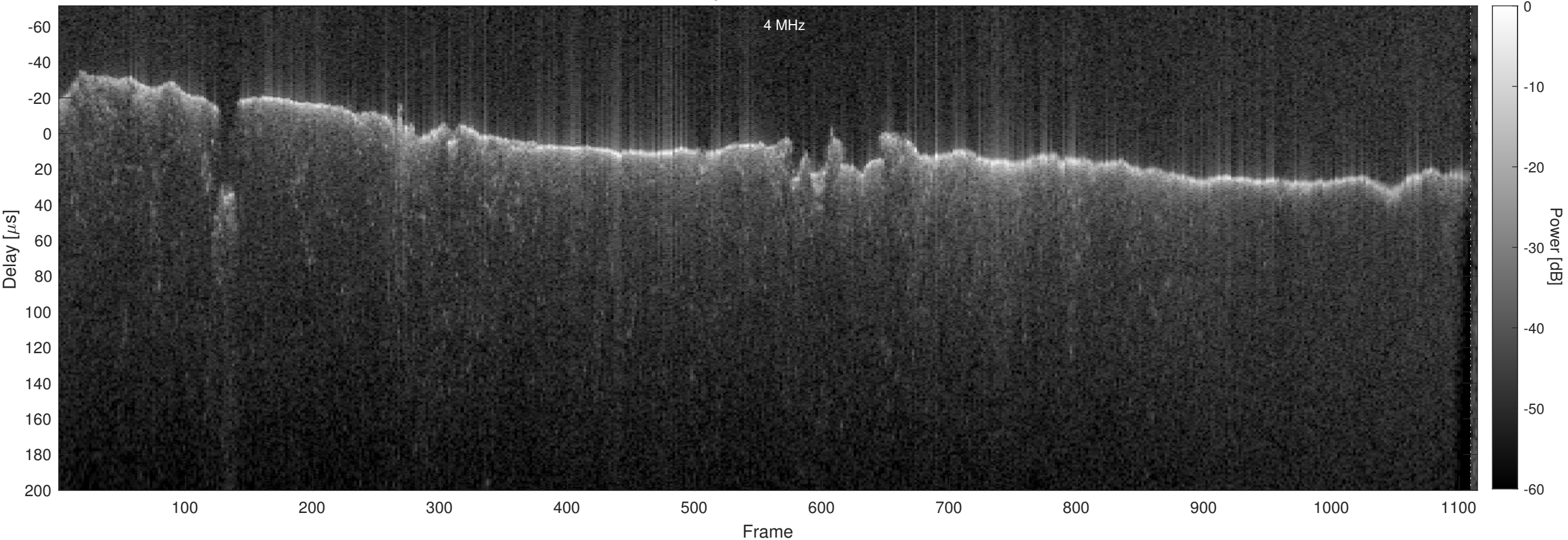
Orbit 22742, Chapman, No Window, Channel 2
