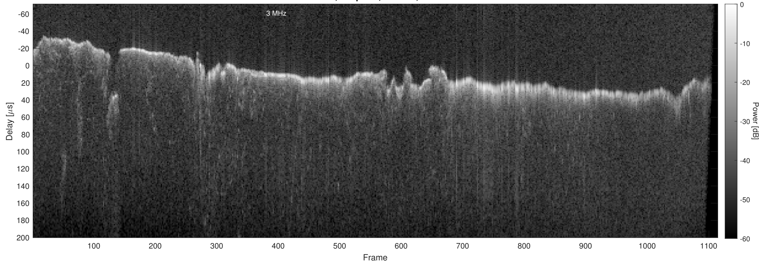
Orbit 22742, Chapman, Window, Channel 2
