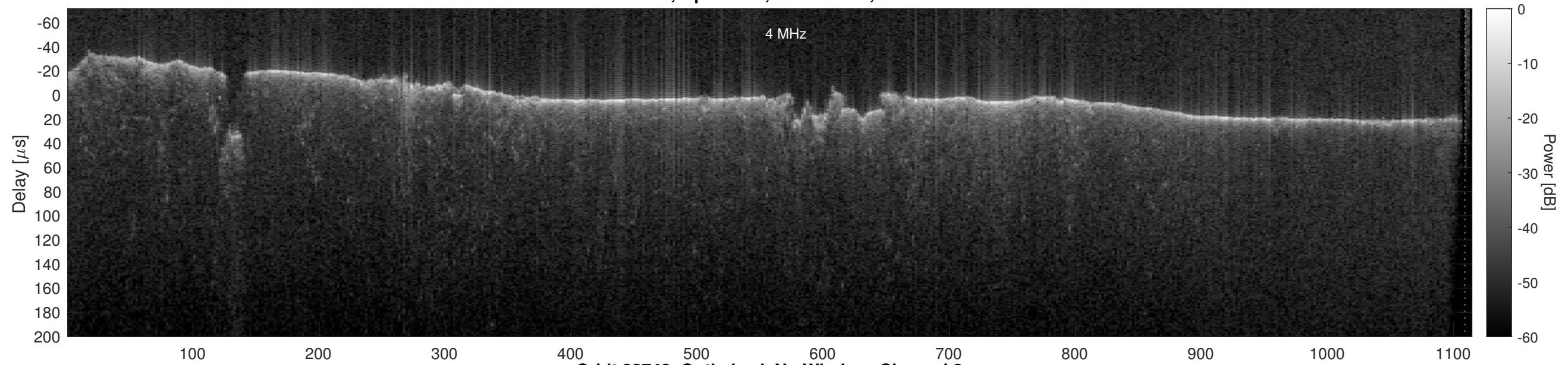
Orbit 22742, Optimized, No Window, Channel 2
