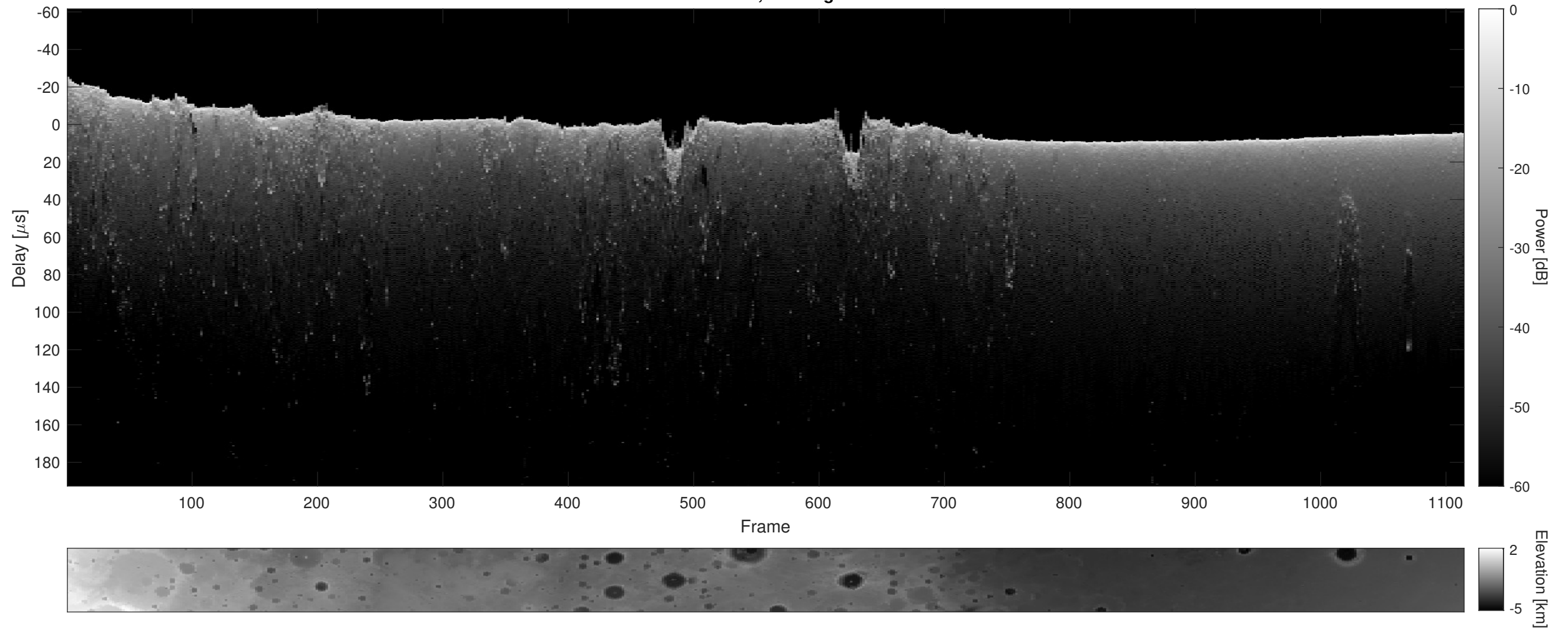
Orbit 22745, Cluttergram
