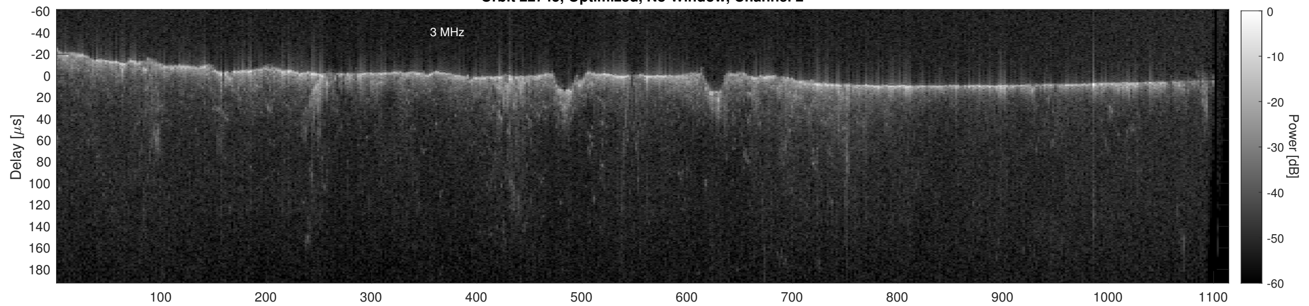
Orbit 22745, Cluttergram
