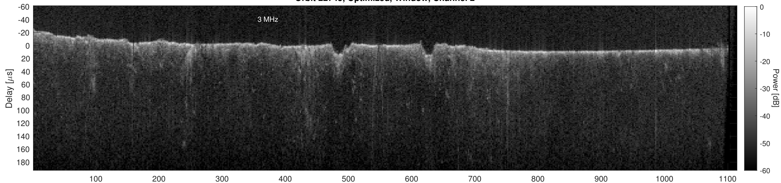
Orbit 22745, Cluttergram
