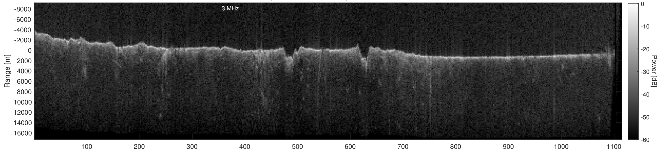
Orbit 22745, Depth-Corrected Cluttergram
