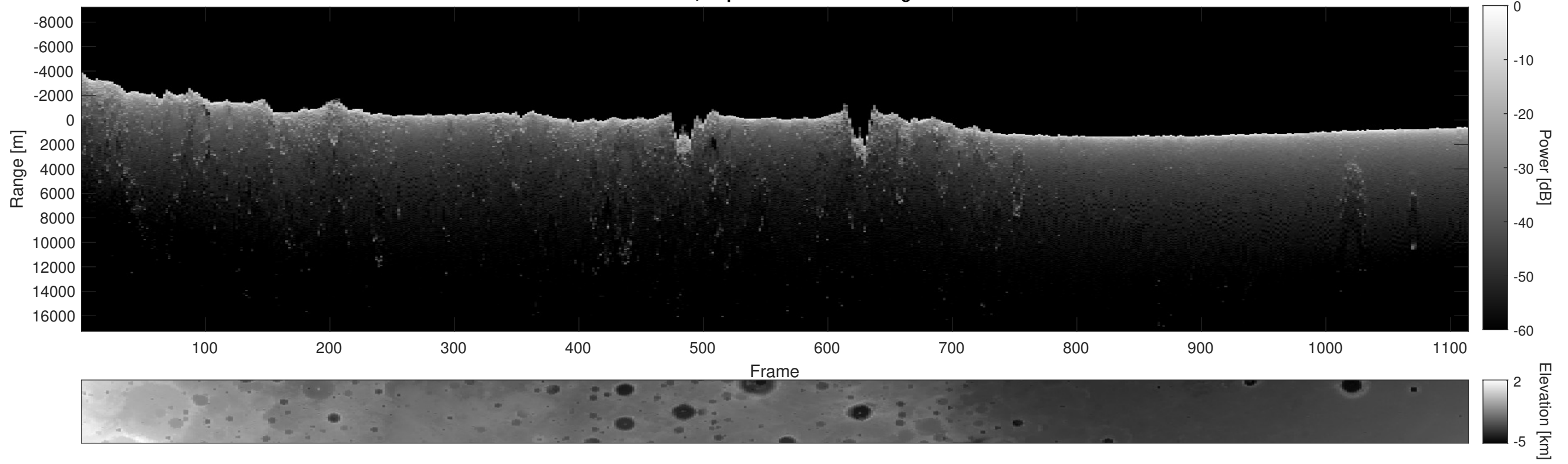
Orbit 22745, Depth-Corrected Cluttergram
