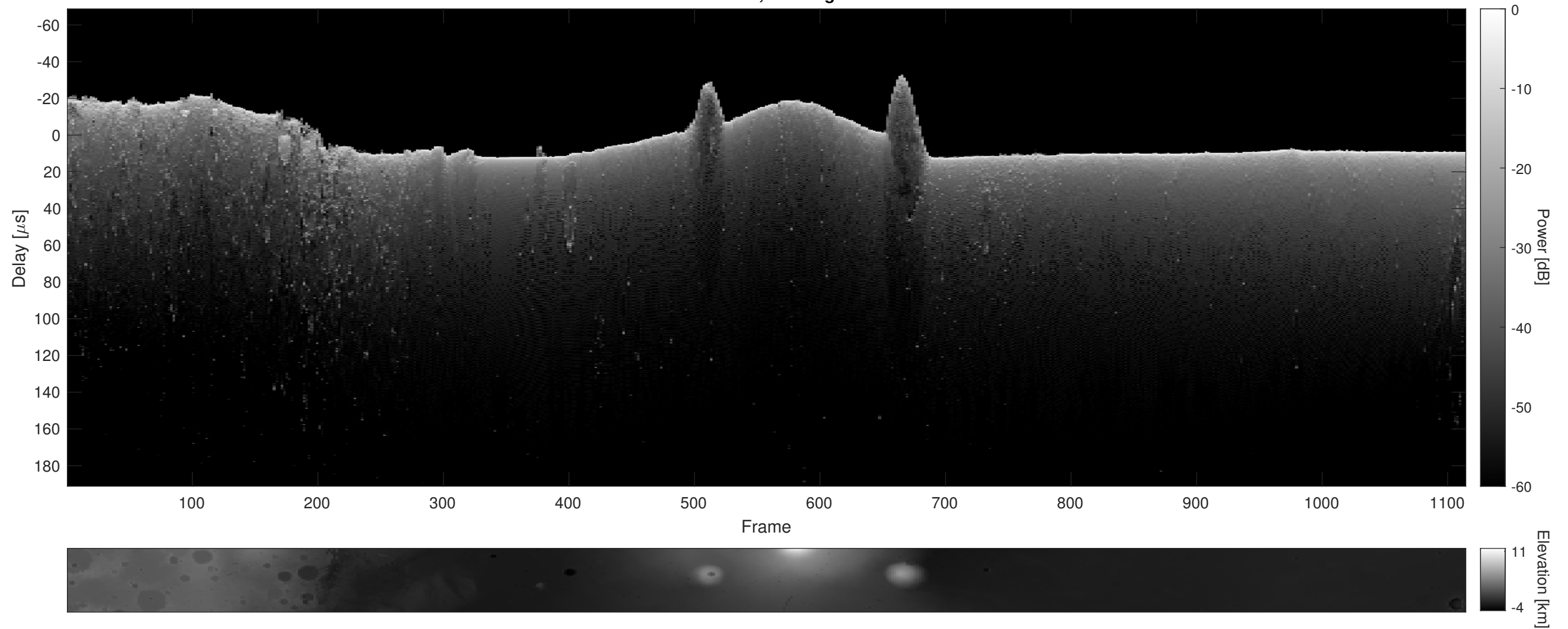
Orbit 22747, Cluttergram
