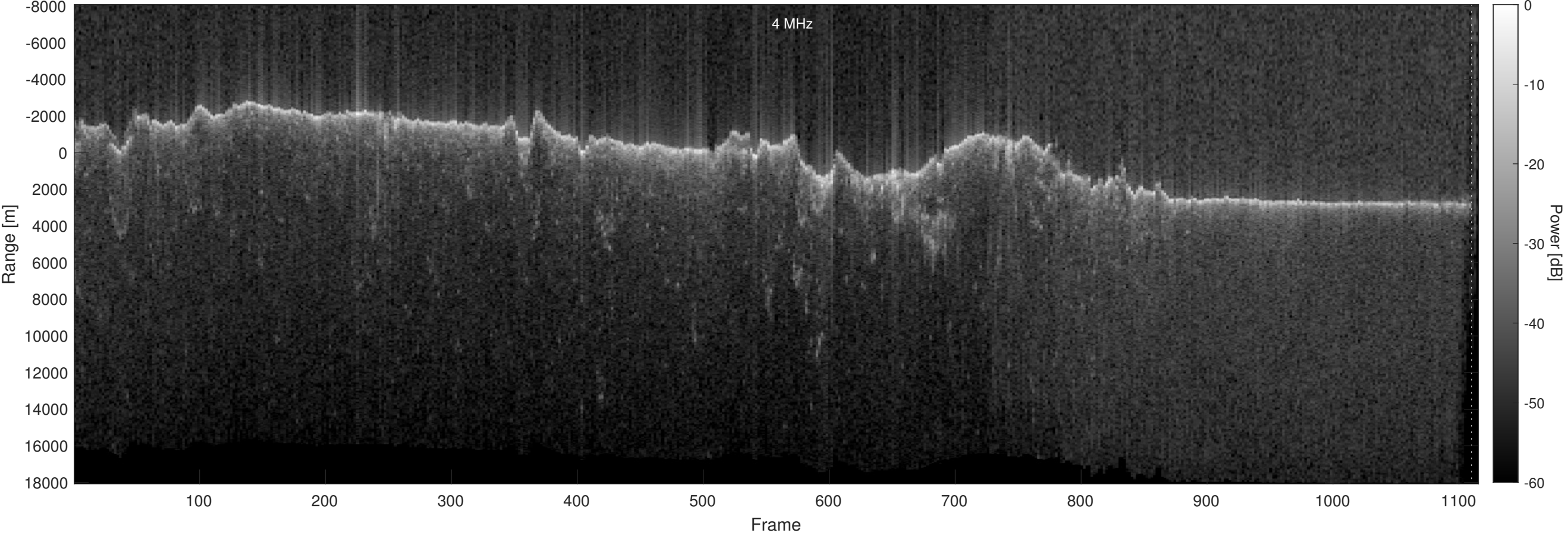
Orbit 22748, Optimized, No Window, Depth-Corrected, Channel 2
