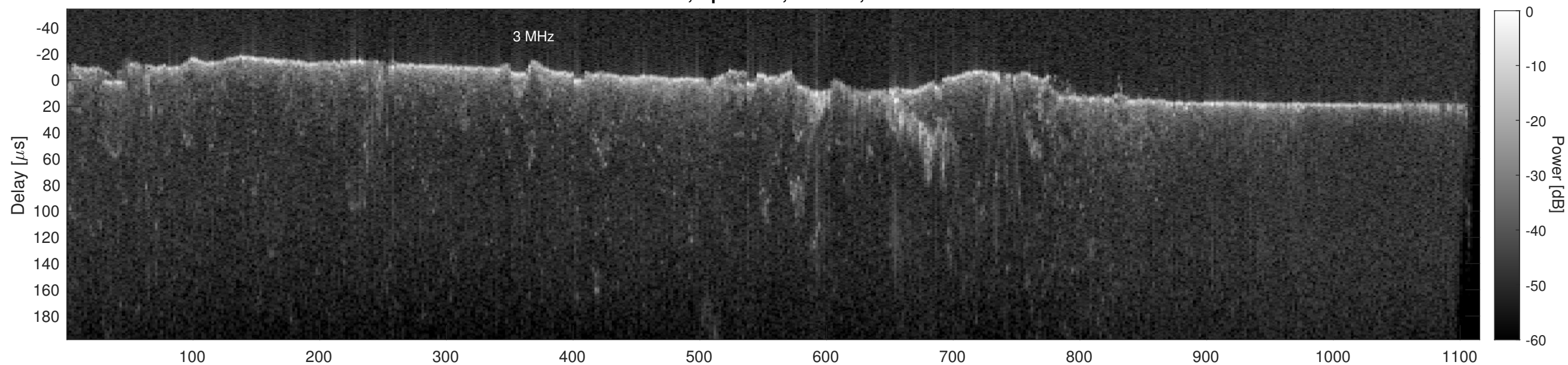
Orbit 22748, Cluttergram
