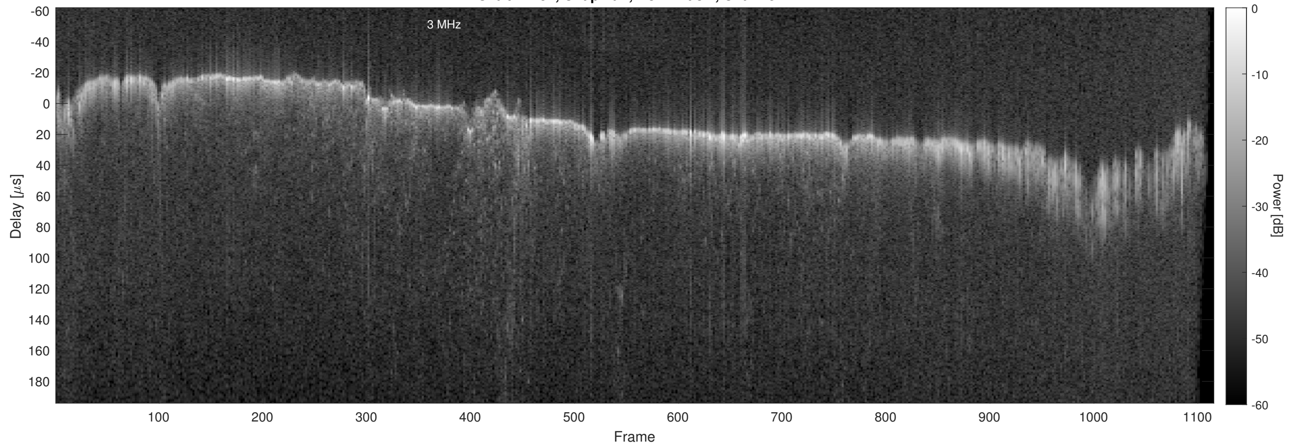
Orbit 22751, Chapman, No Window, Channel 2
