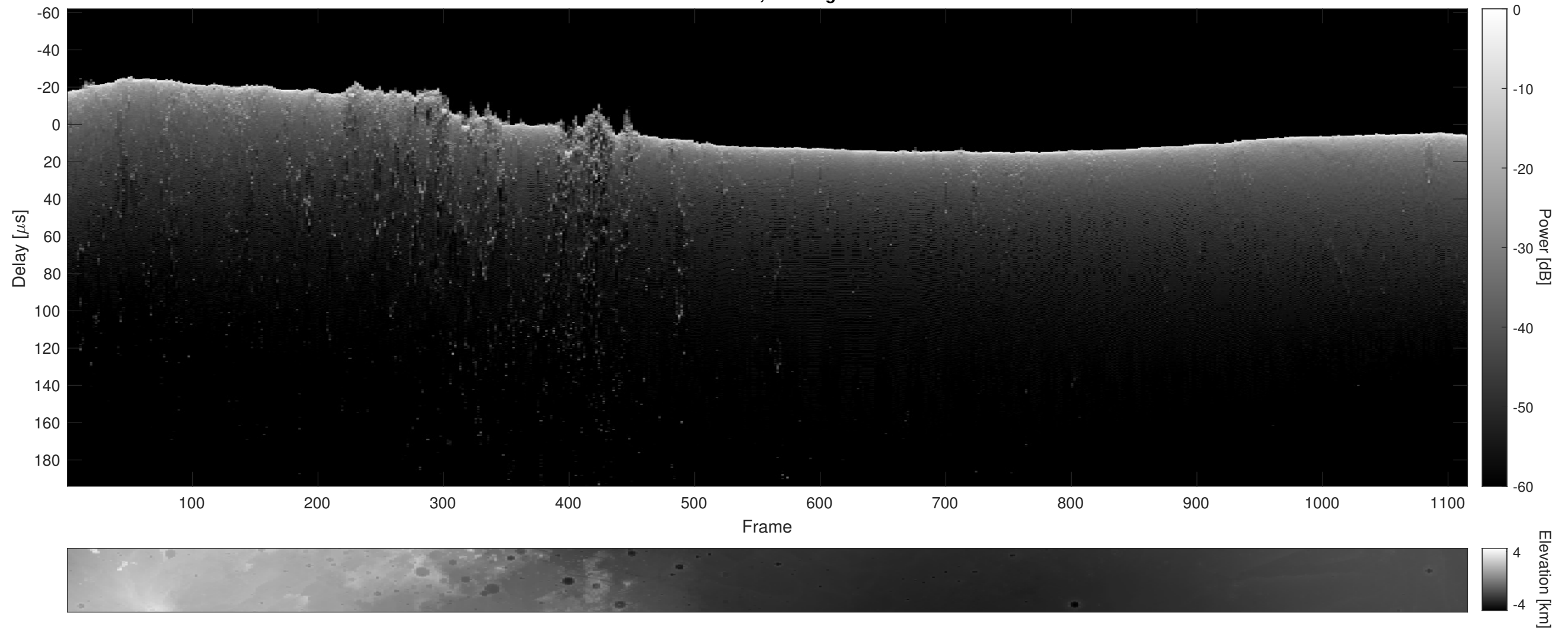
Orbit 22751, Cluttergram
