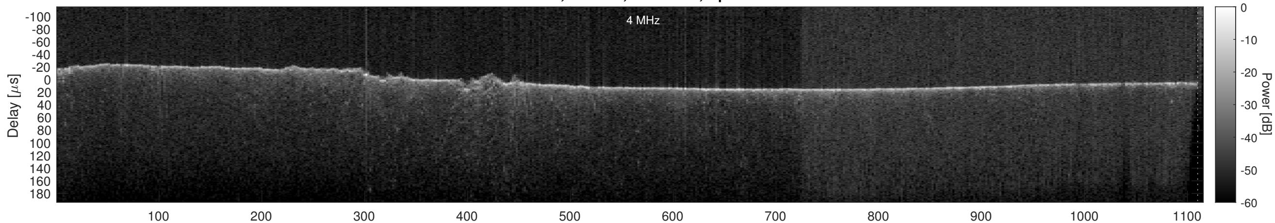
Orbit 22751, Cluttergram
