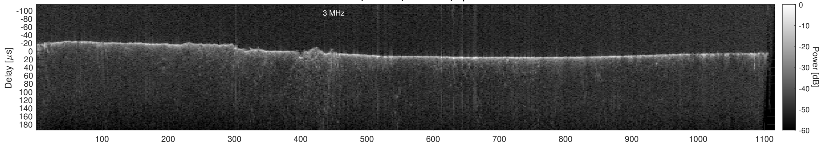
Orbit 22751, Cluttergram
