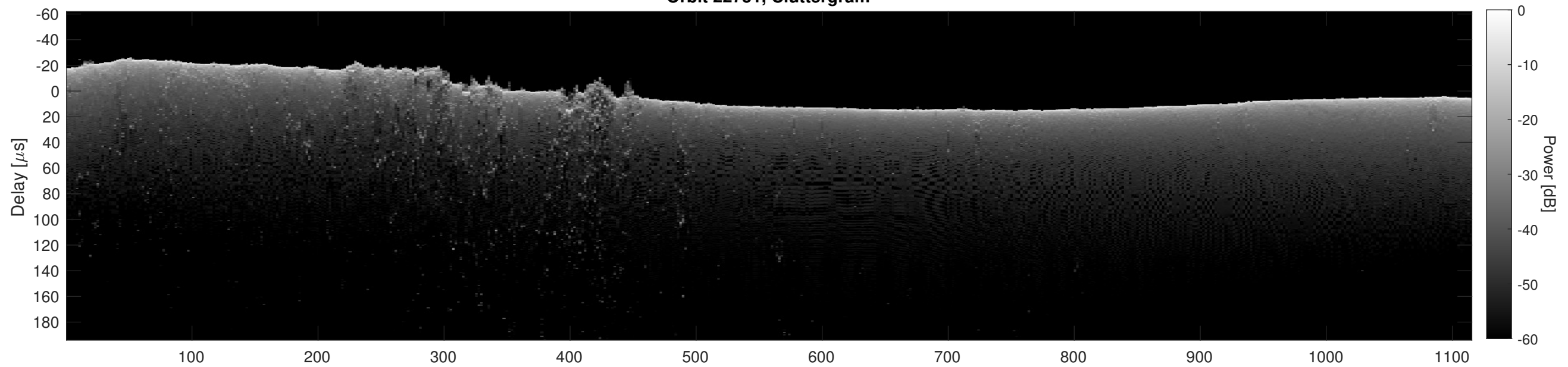
Orbit 22751, Cluttergram
