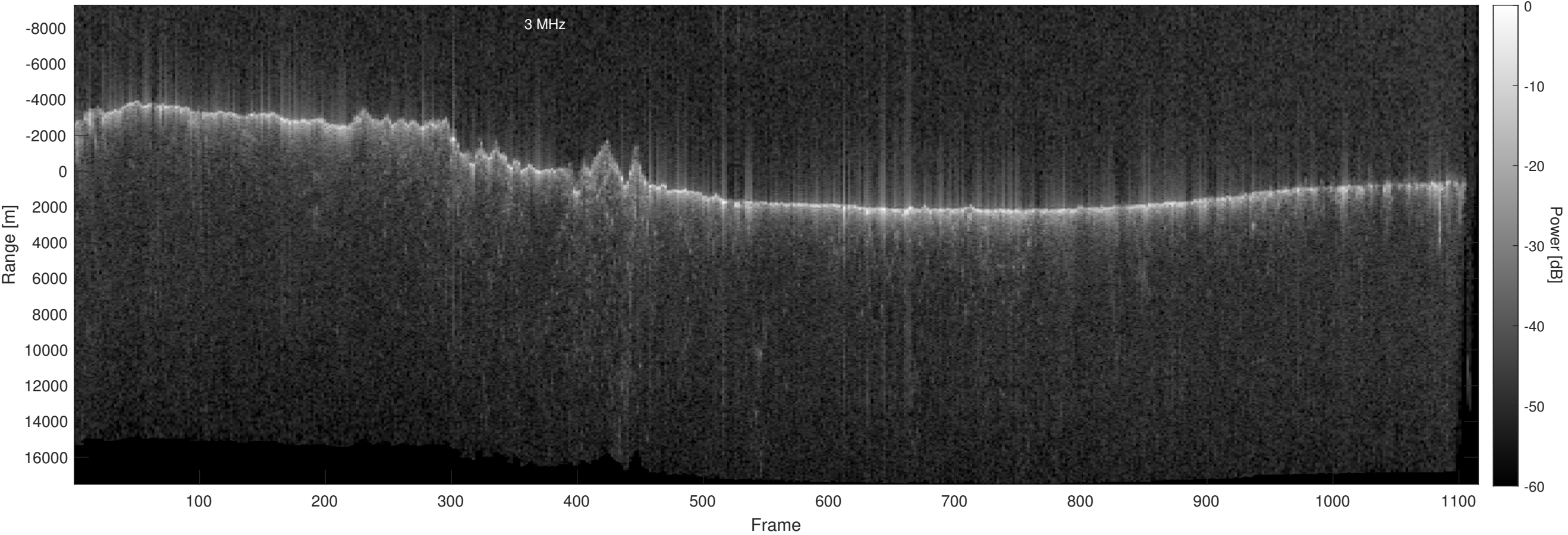
Orbit 22751, Optimized, No Window, Depth-Corrected, Channel 2
