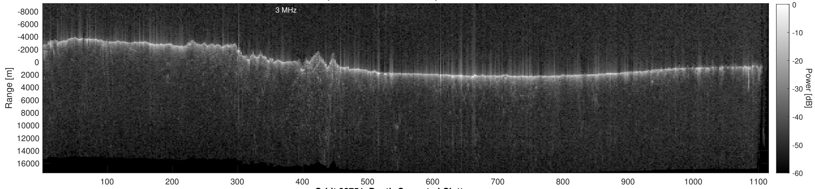
Orbit 22751, Depth-Corrected Cluttergram
