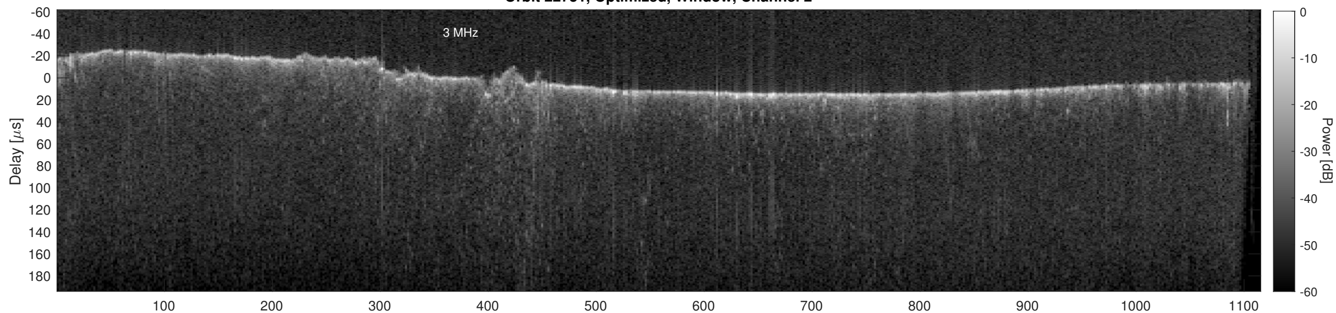
Orbit 22751, Cluttergram
