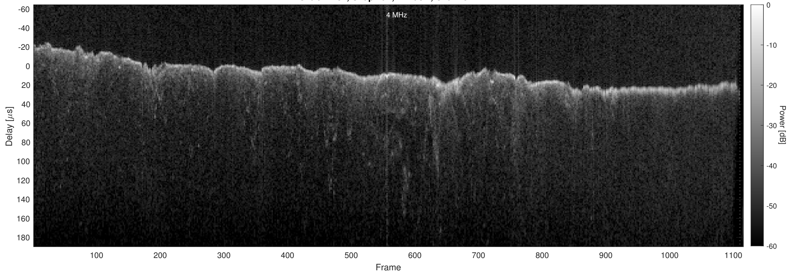
Orbit 22752, Chapman, Window, Channel 2
