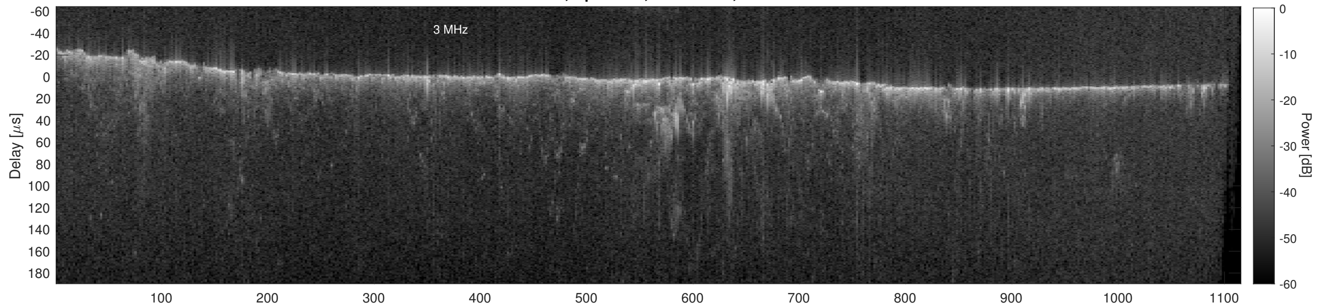
Orbit 22752, Cluttergram
