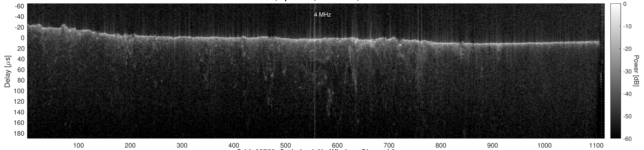
Orbit 22752, Optimized, No Window, Channel 2
