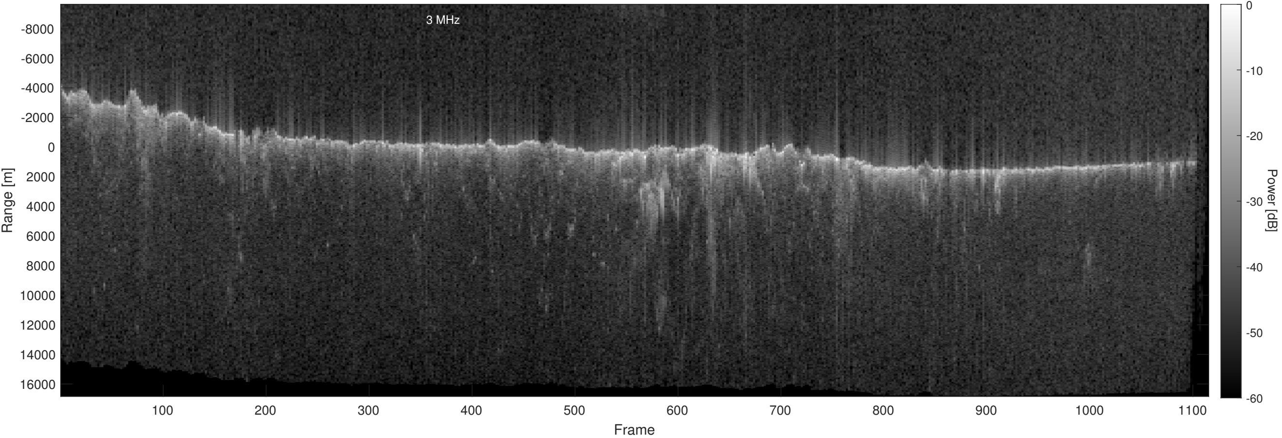
Orbit 22752, Optimized, No Window, Depth-Corrected, Channel 2
