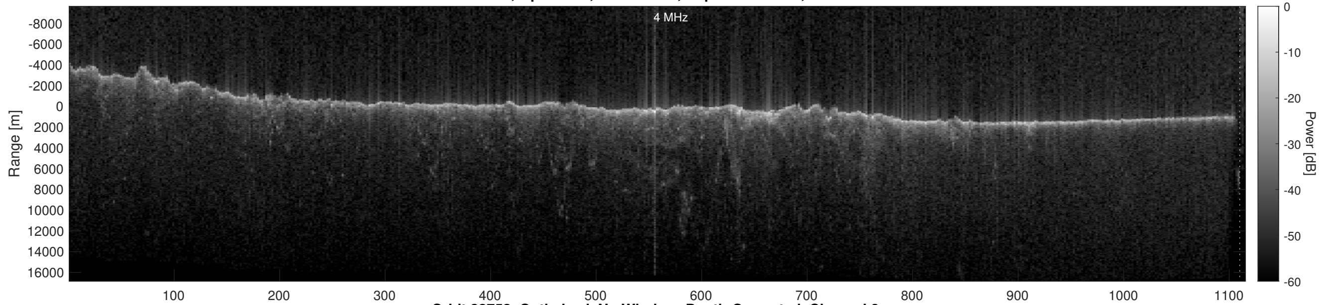
Orbit 22752, Optimized, No Window, Depth-Corrected, Channel 2
