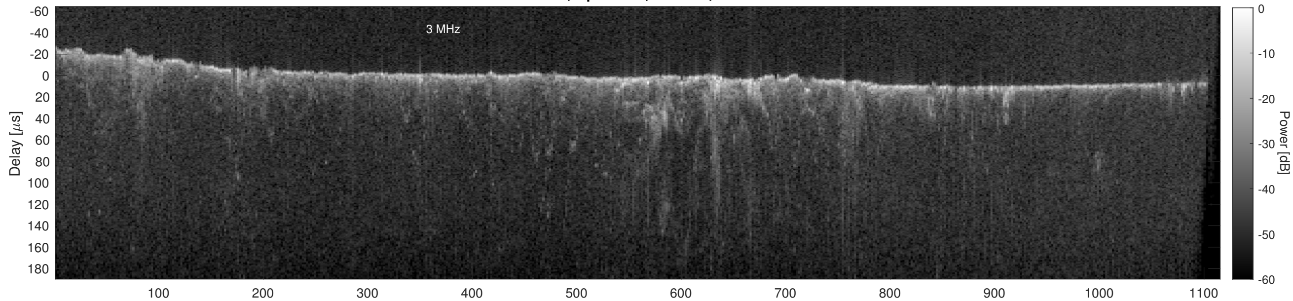
Orbit 22752, Cluttergram
