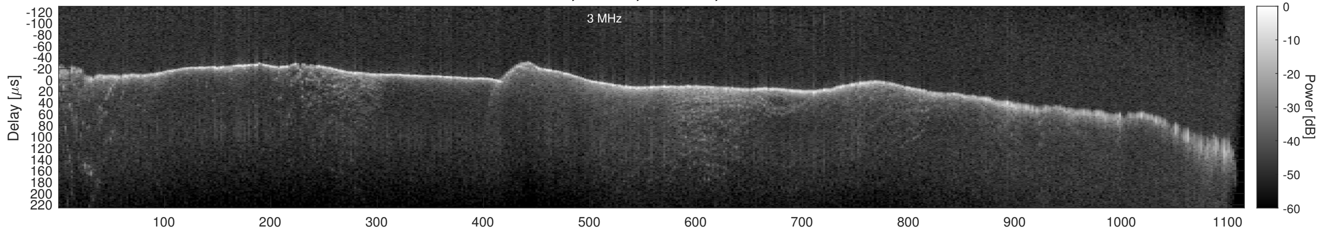
Orbit 22753, Window, Channel 2, Chapman
