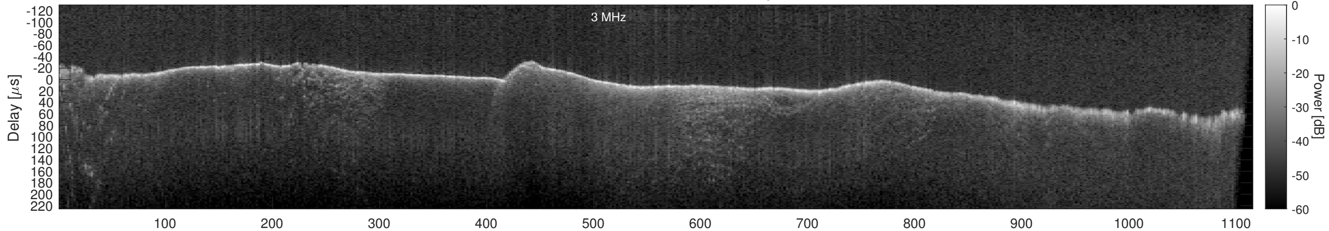
Orbit 22753, Window, Channel 2, Optimized
