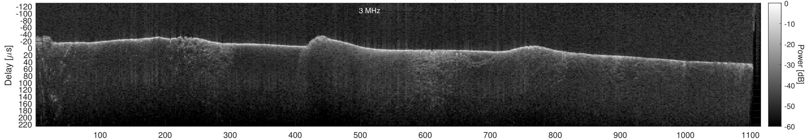
Orbit 22753, Cluttergram
