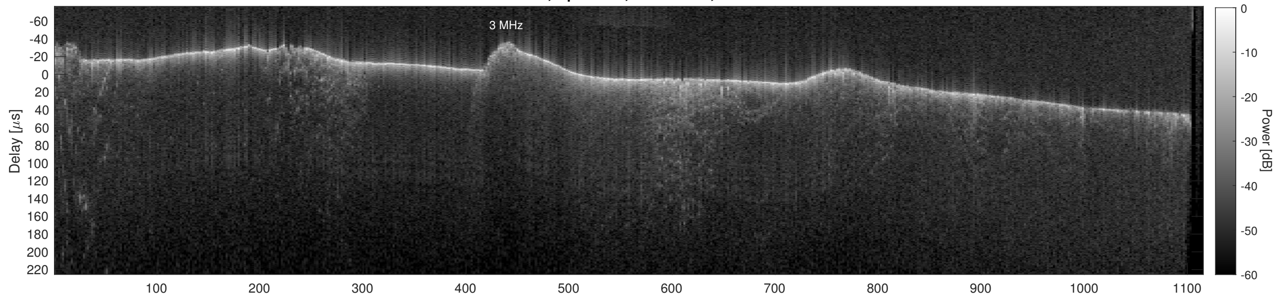
Orbit 22753, Cluttergram
