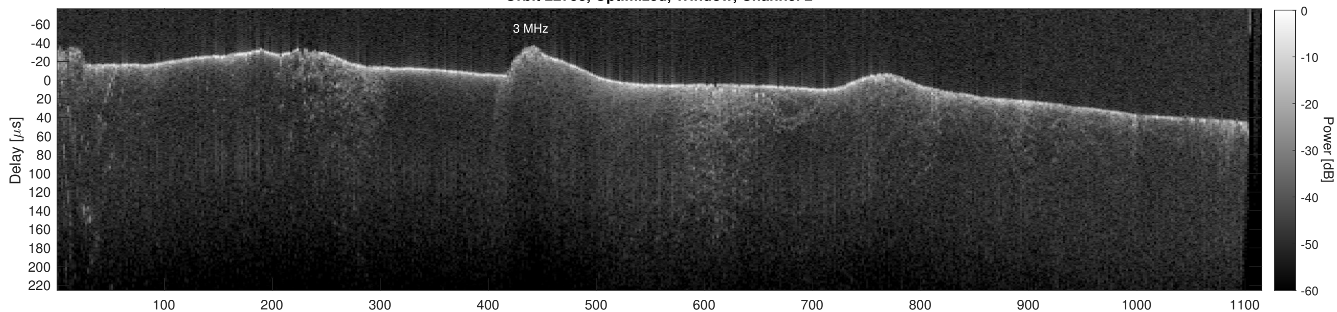
Orbit 22753, Cluttergram
