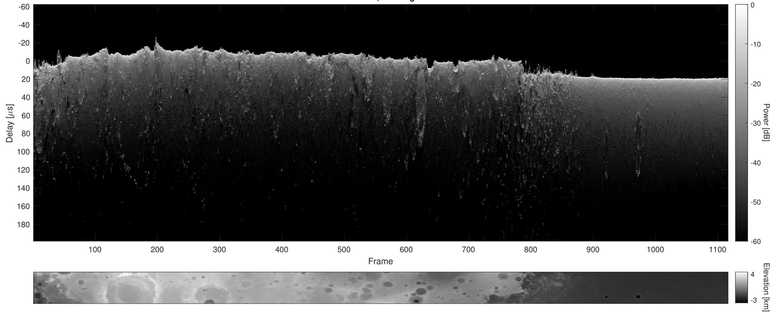
Orbit 22755, Cluttergram
