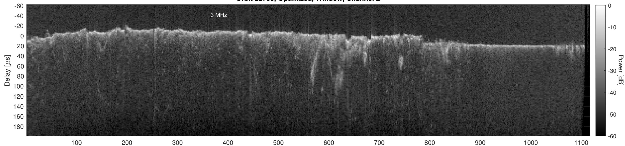
Orbit 22755, Cluttergram
