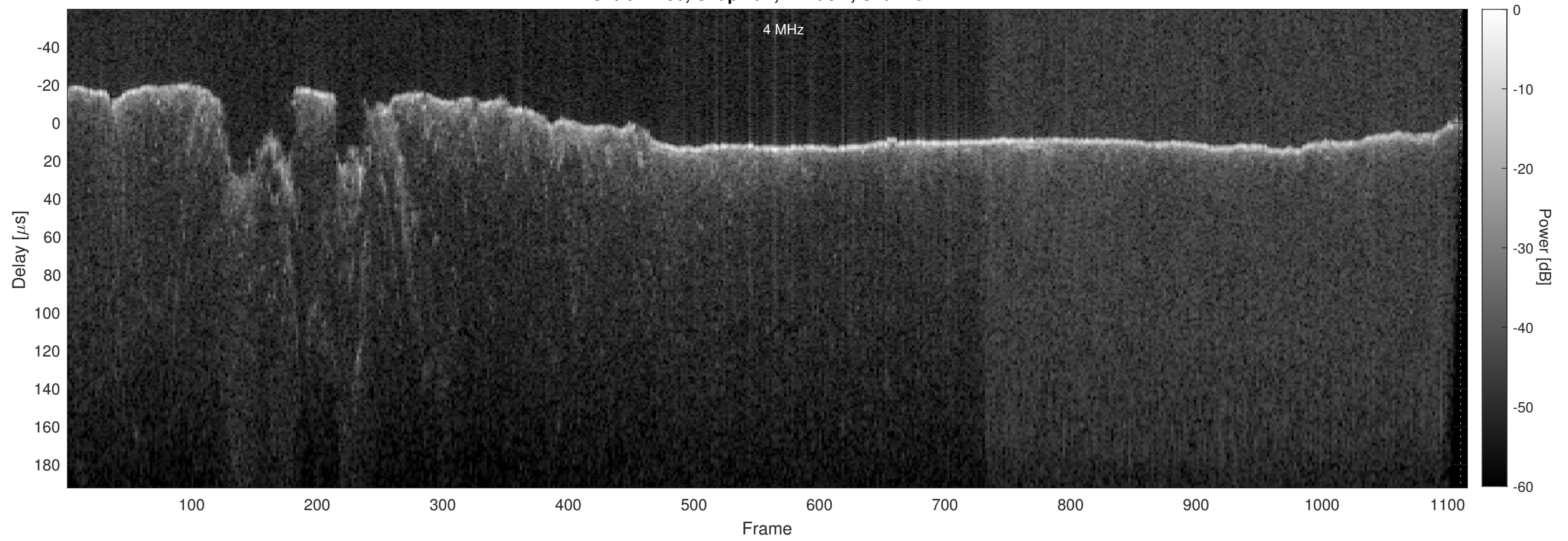
Orbit 22756, Chapman, Window, Channel 2
