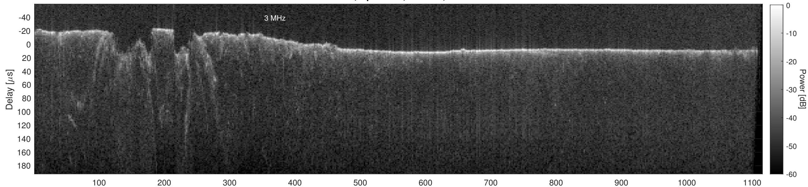
Orbit 22756, Cluttergram
