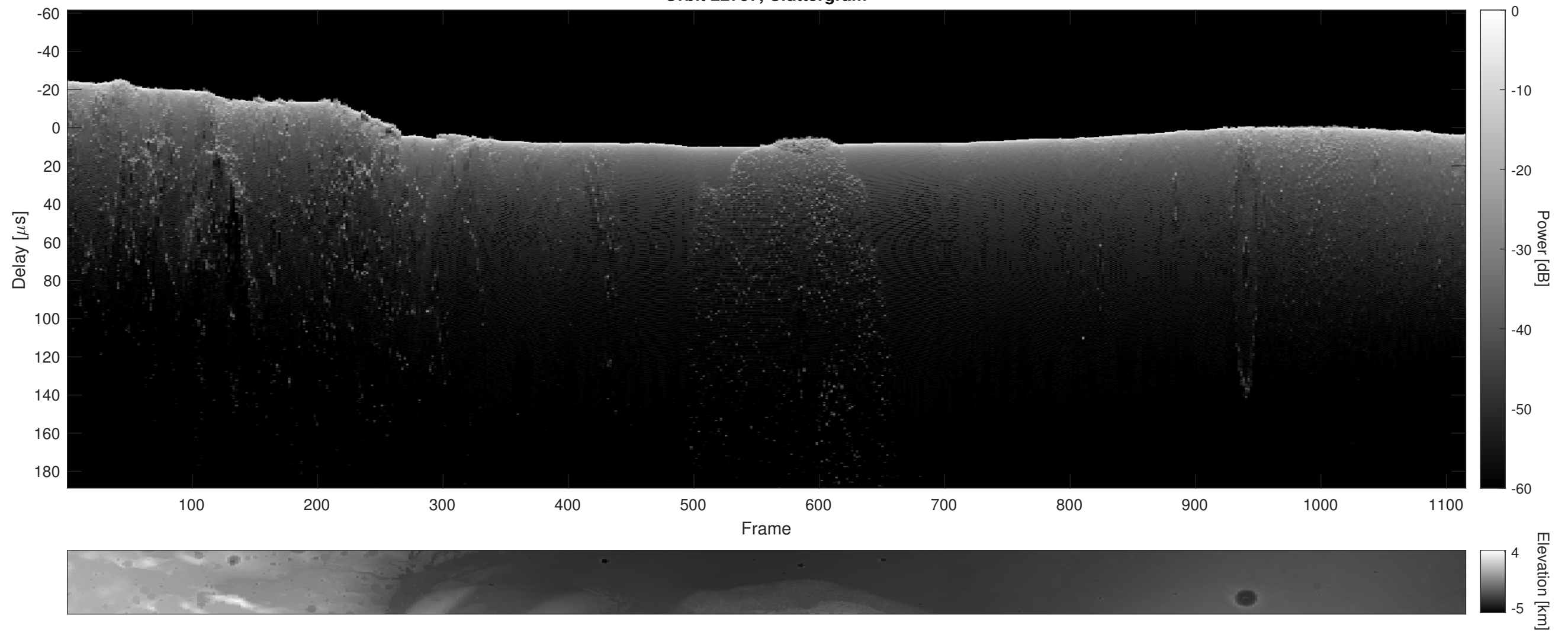
Orbit 22757, Cluttergram
