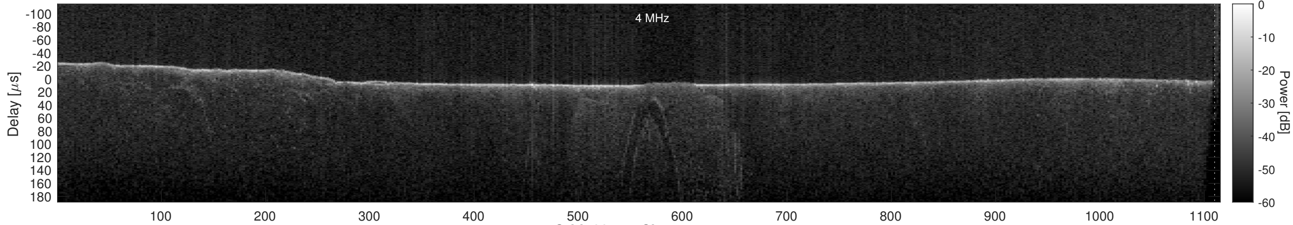
Orbit 22757, Cluttergram
