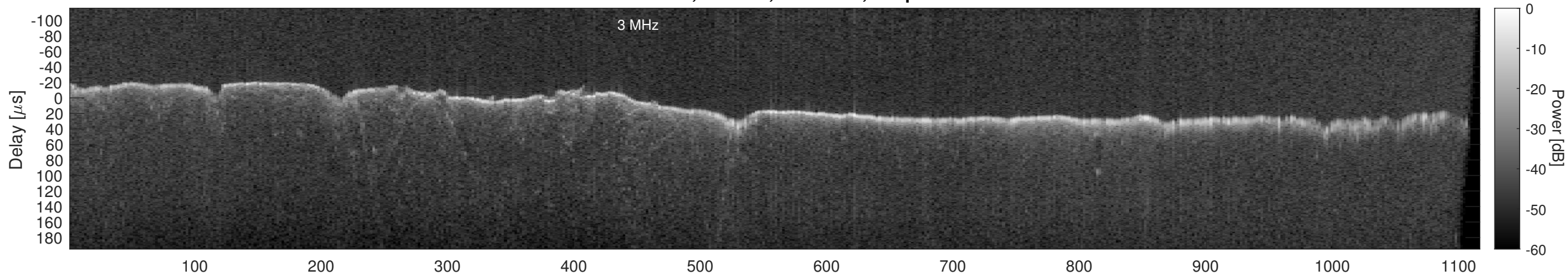
Orbit 22758, Window, Channel 2, Optimized
