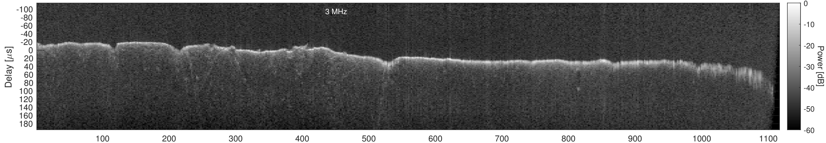
Orbit 22758, Window, Channel 2, Chapman
